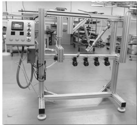
PNEUMATIC TEST STAND
