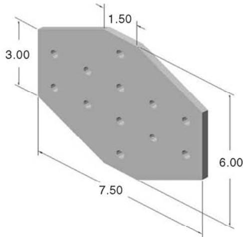
Part Wt: .850 lbs
