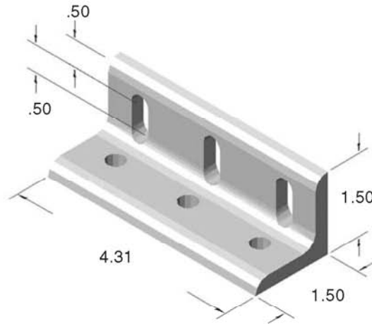
Part Wt: .265 lbs
