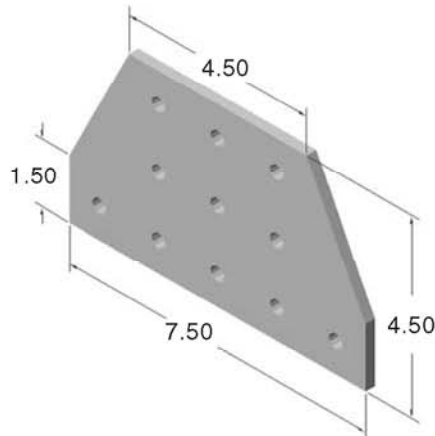
Part Wt: .680 lbs
