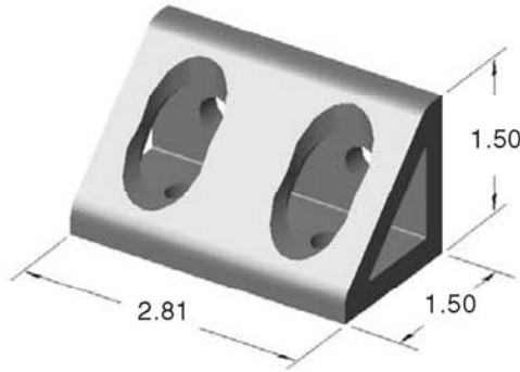
Part Wt: .245 lbs
