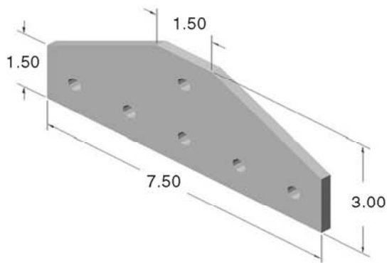
Part Wt: .415 lbs
