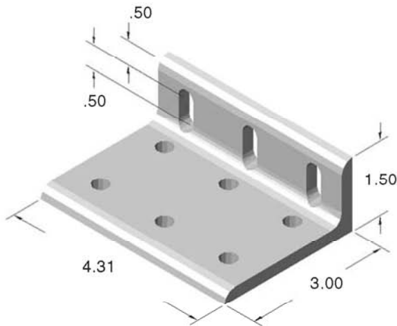
Part Wt: .410 lbs
